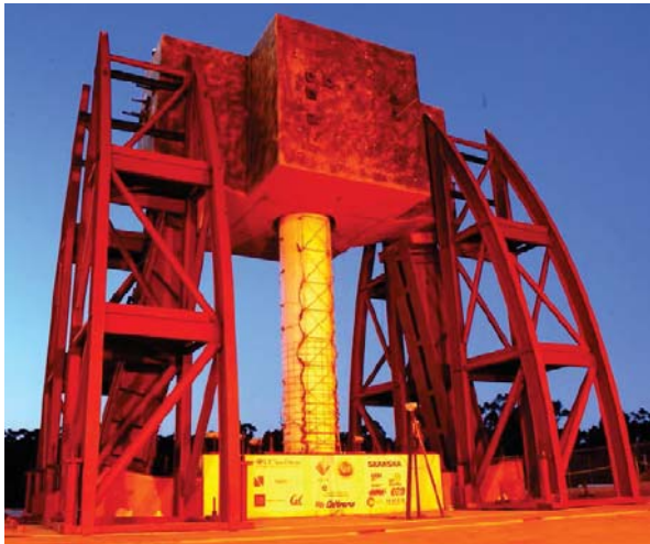
Fig. 3 Test set-up [12]
